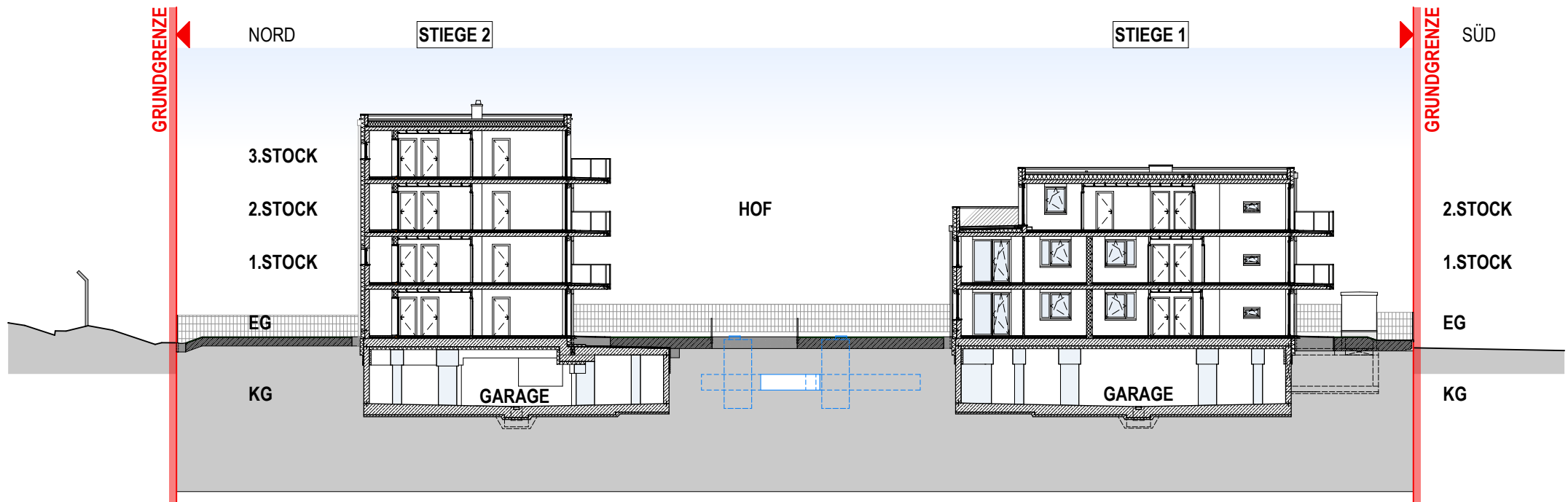
SCHNITT 4-4 M = 1:300
